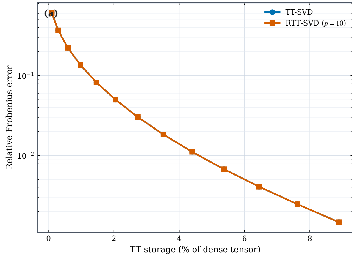
Accuracy at a fixed storage budget
