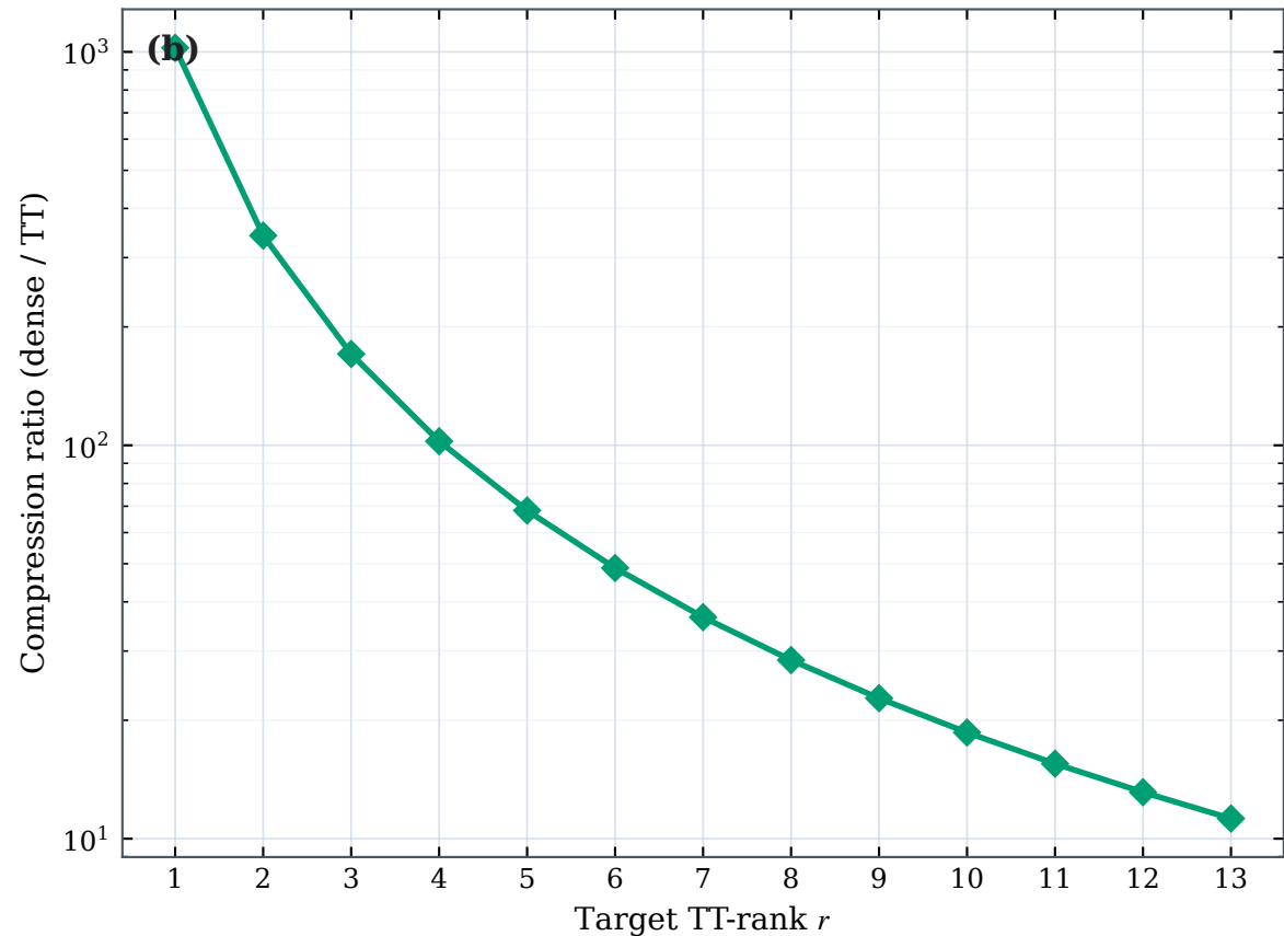
Compression versus target rank
