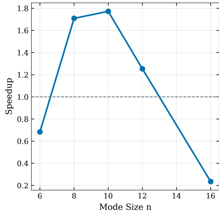
Speedup vs Mode Size
