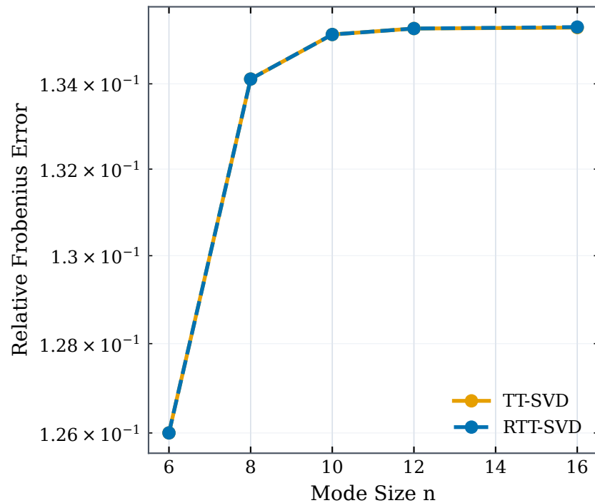
Approximation Error vs Mode Size
