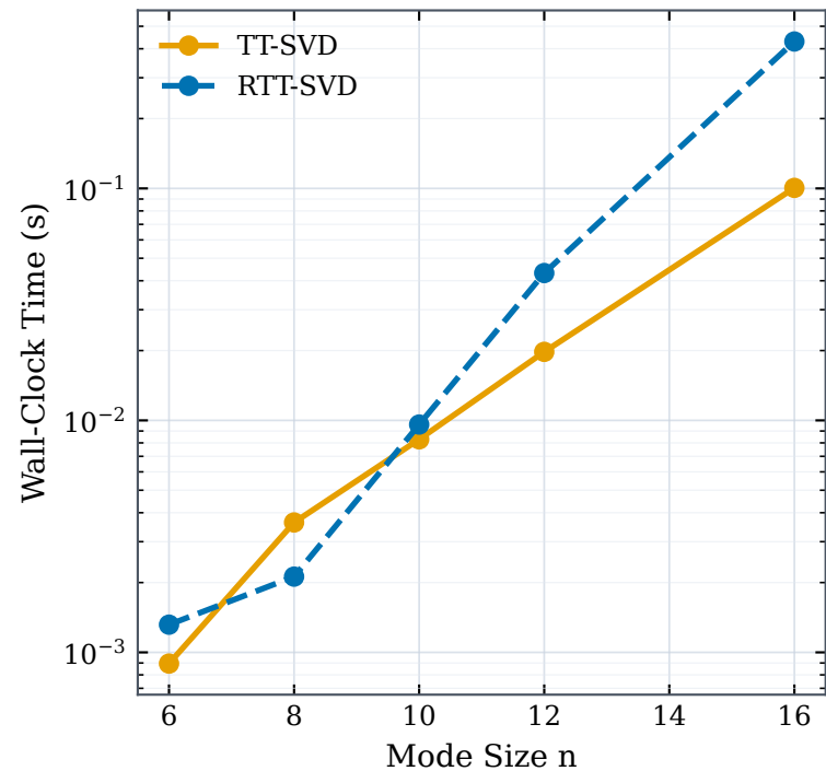
Computation Time vs Mode Size
