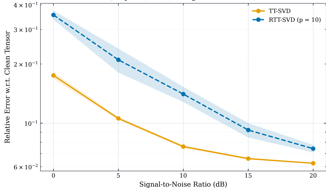
Noise Robustness: RTT-SVD vs TT-SVD (shape 12^4 , r = 4 , averaged over 10 trials)
