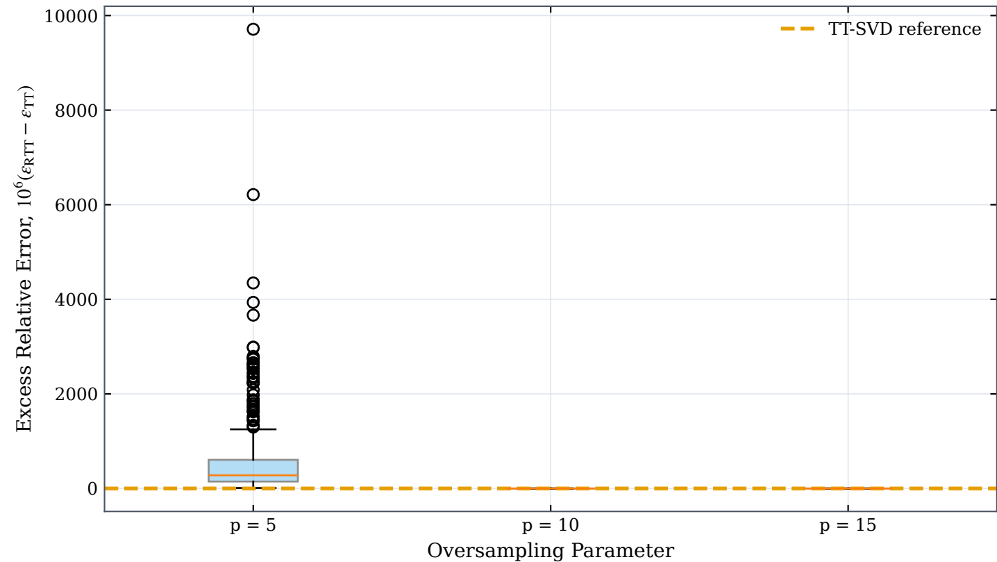
RTT-SVD Error Concentration over 500 Random Trials (shape 12^4 , r = 5 )
