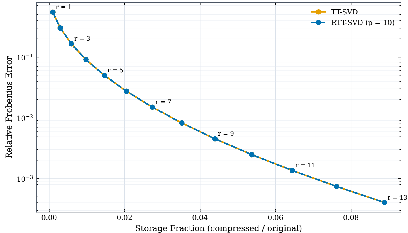
Storage-Accuracy Trade-off (Pareto Front) (shape 16^4 , exponential decay)
