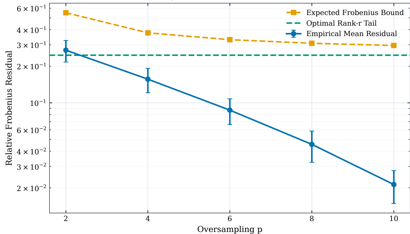
Gaussian Range-Finder Residual vs Expected Bound (first unfolding of shape 32 \times 16^3 , r = 4 , 200 trials per p )
