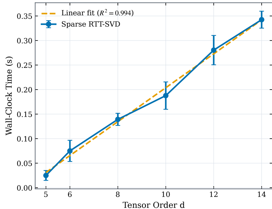
Sparse RTT-SVD Runtime vs Tensor Order
