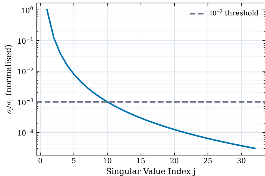
Polynomial ( \beta = 3.0 )
