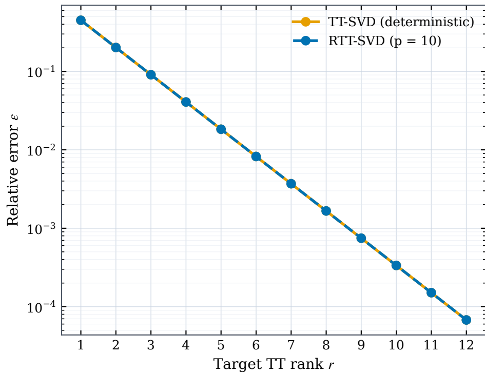
Exponential decay ( \alpha = 0.8 )
