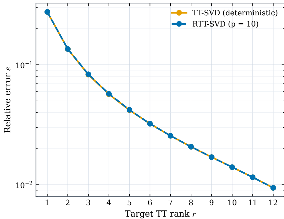
Polynomial decay ( \beta = 2.0 )
