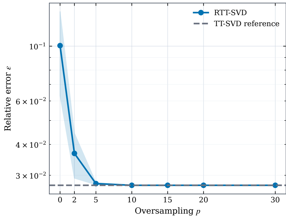
Relative error as a function of p
