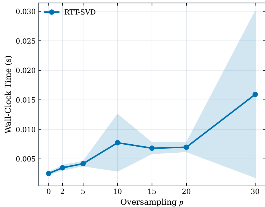
Runtime as a function of p
