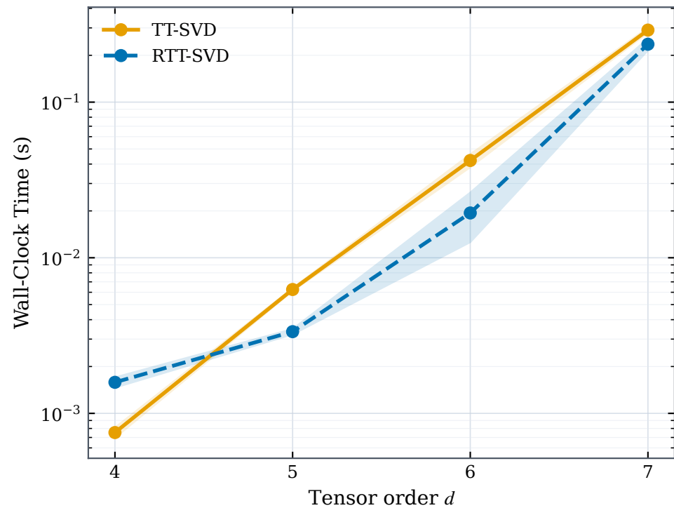
Runtime as a function of tensor order d
