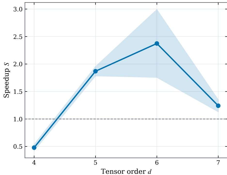
Speedup as a function of d
