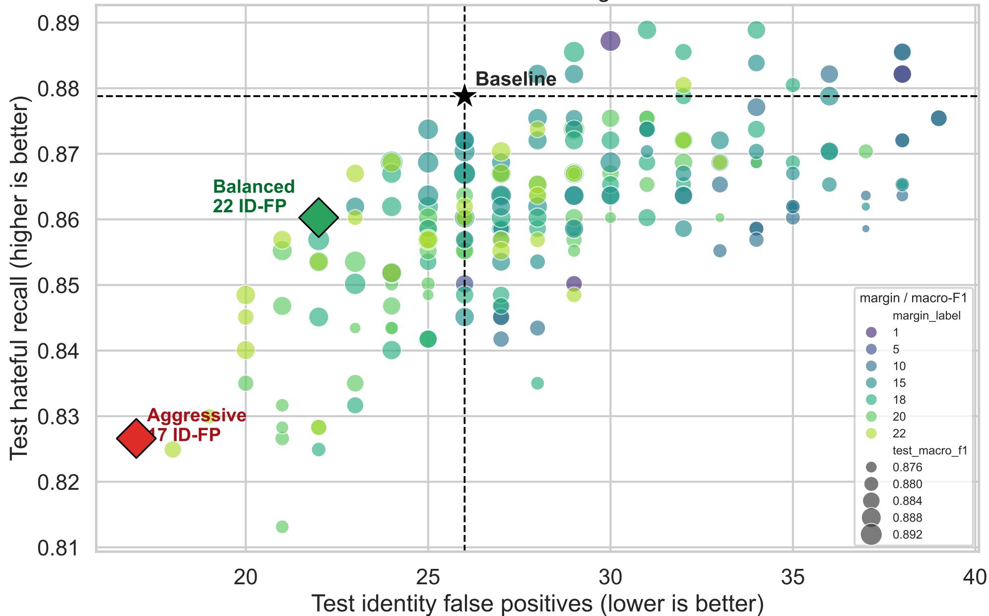
Contrastive Fine-Tuning Trade-Off
