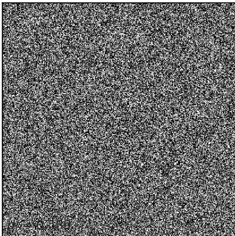
critical ( b = b_c = 0.126 )
