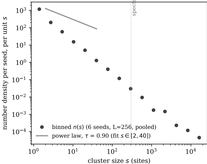
Cluster-size distribution at b \approx b_c = 0.126 (L=256)
