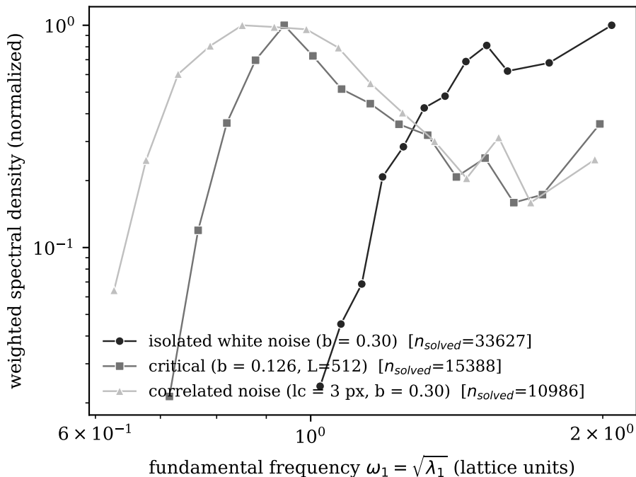
Dirichlet cavity spectra across the three regimes
