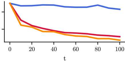
Cross-Entropy
