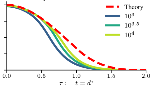
Frequencies from Real Data
