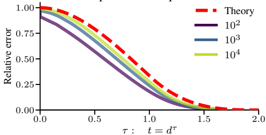
Zipf's Law Frequencies
