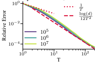
Synthetic Data, Transition
