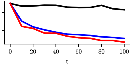
Cross-Entropy
