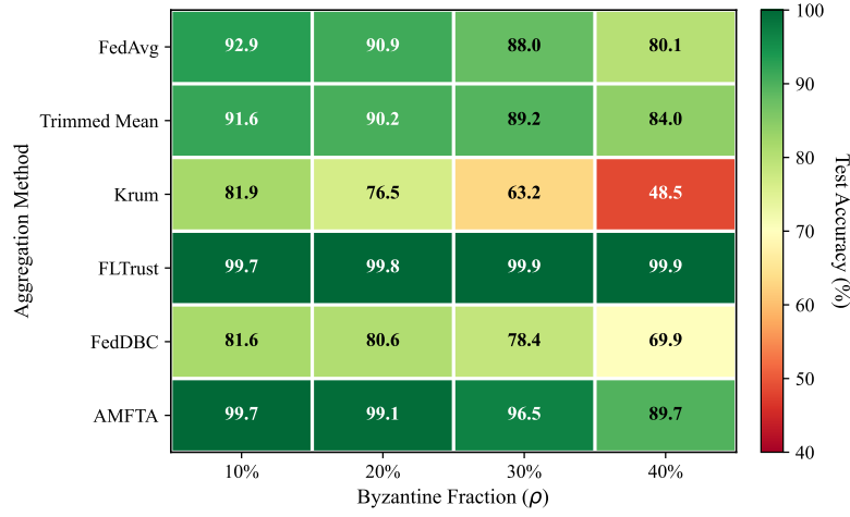
Fig. 9 Accuracy heatmap under Label Flipping attacks. Each cell shows the mean test accuracy (%) averaged over 5 seeds. Red cells indicate catastrophic degradation; green cells indicate robust performance.
