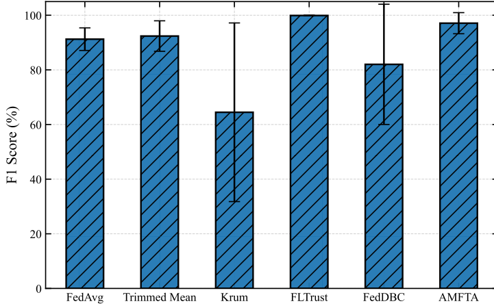
Fig. 7 F1 Score under Label Flipping at \rho = 0.30 .
