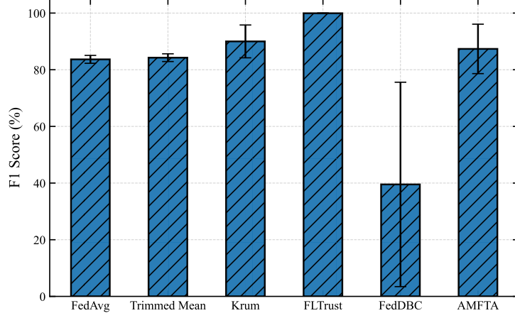
Fig. 8 F1 Score under Gaussian Noise at \rho = 0.30 .
