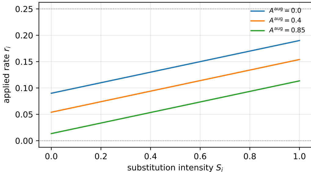
Rate function: bounded and monotone (Proposition 3)
