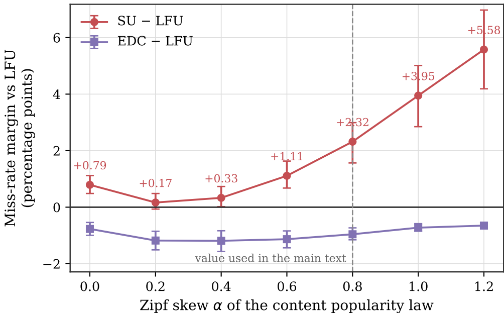
Demand-model sensitivity (synthetic tier, 10 seeds) at \alpha = 0 popularity carries no rank information
