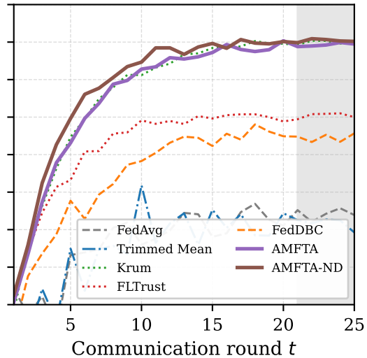
Gaussian noise ( \rho = 0.30 )
