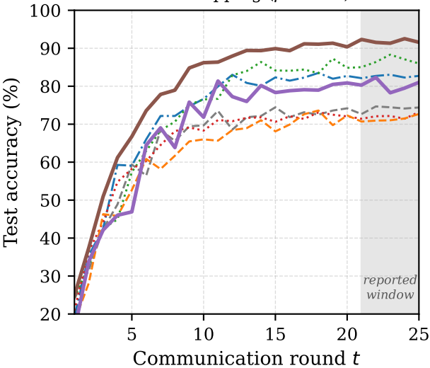
Label flipping ( \rho = 0.30 )
