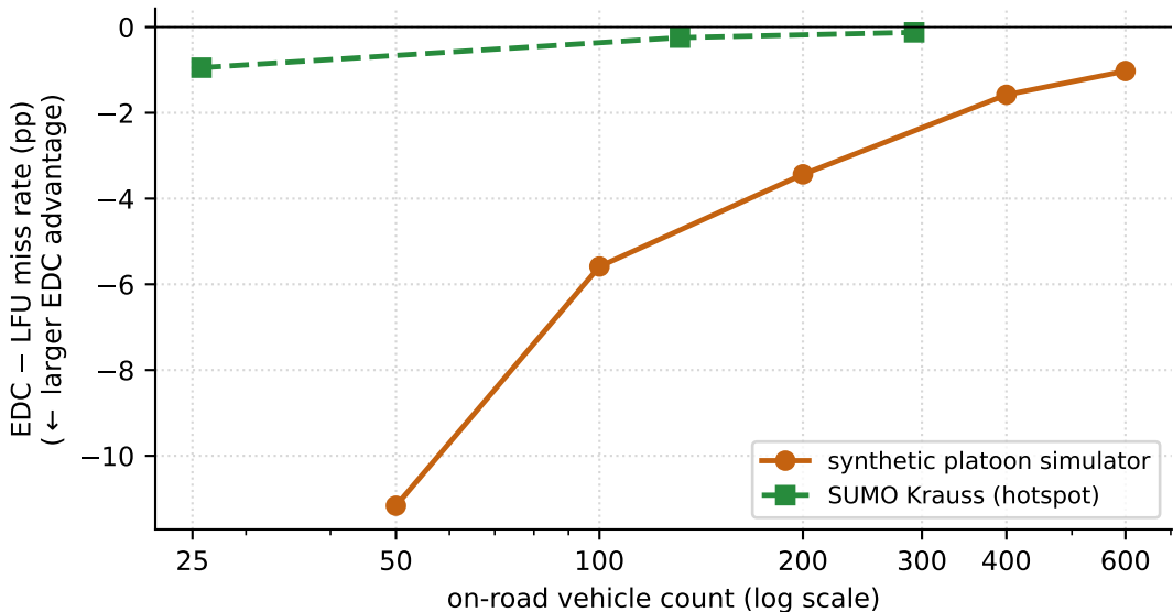
Synthetic platoon model overstates EDC's spatial advantage (margins 3-10× larger than under realistic SUMO traffic)
