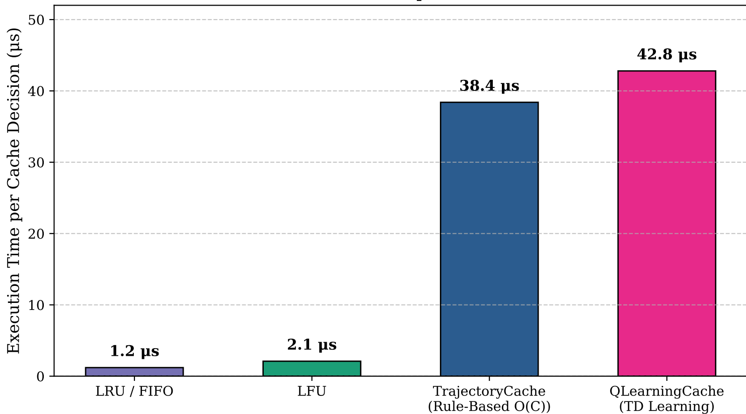
Wall-Clock Inference Overhead per Cache Eviction Decision
