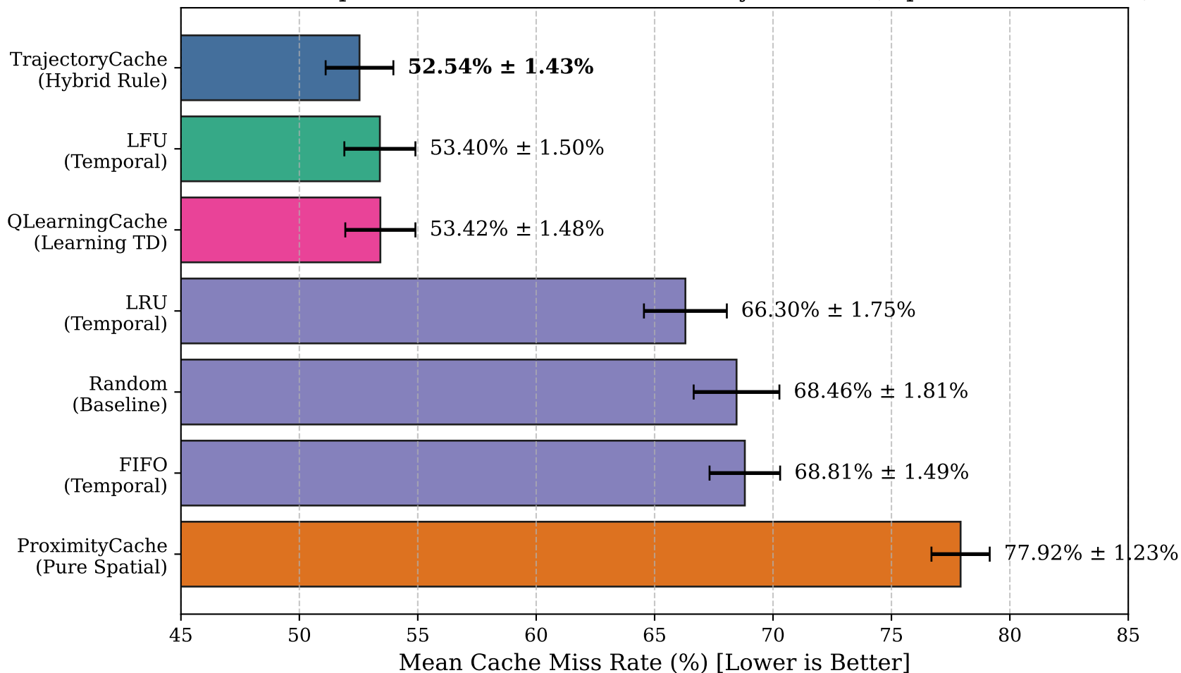
Extended Comparative Evaluation Across Policy Families (Zipf \alpha=0.8 , 10 Seeds)
