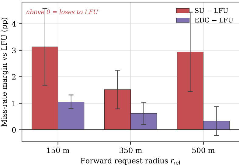
Free-flow real traffic (US-101, 41 km/h, 10 seeds): SU loses to LFU at every radius
