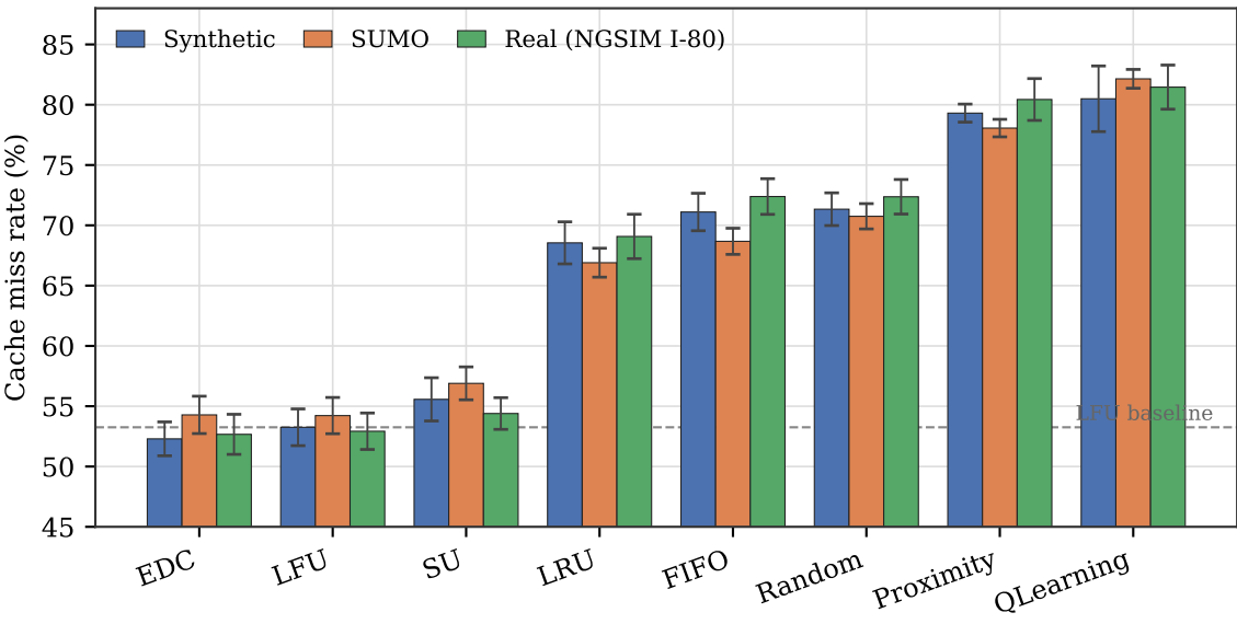
Controlled configuration (535 m, r_{\text{rel}} = 150 m), 10 seeds; lower is better
