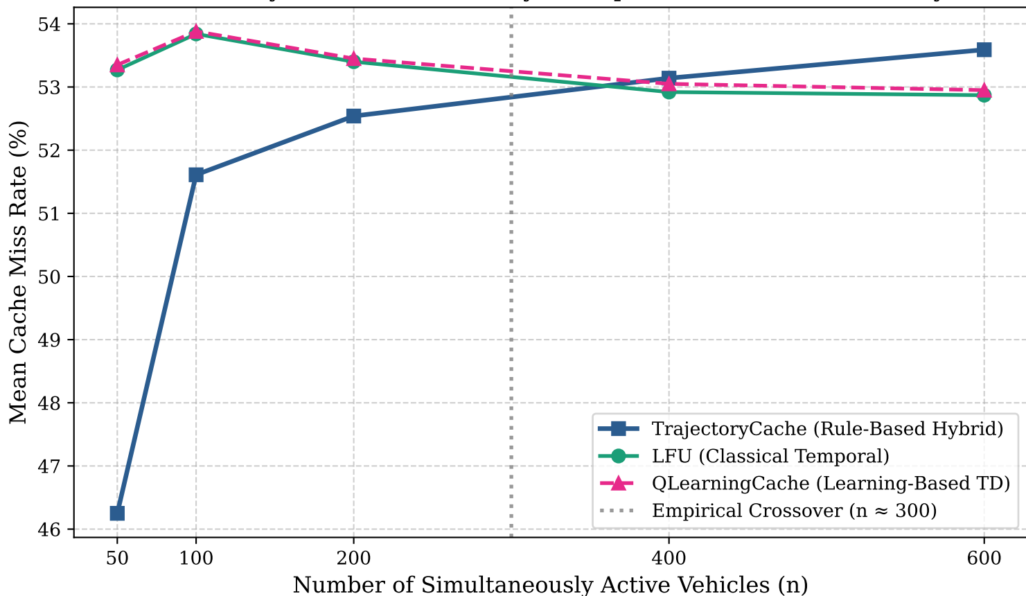
Sensitivity to Vehicular Density & Empirical Crossover Boundary
