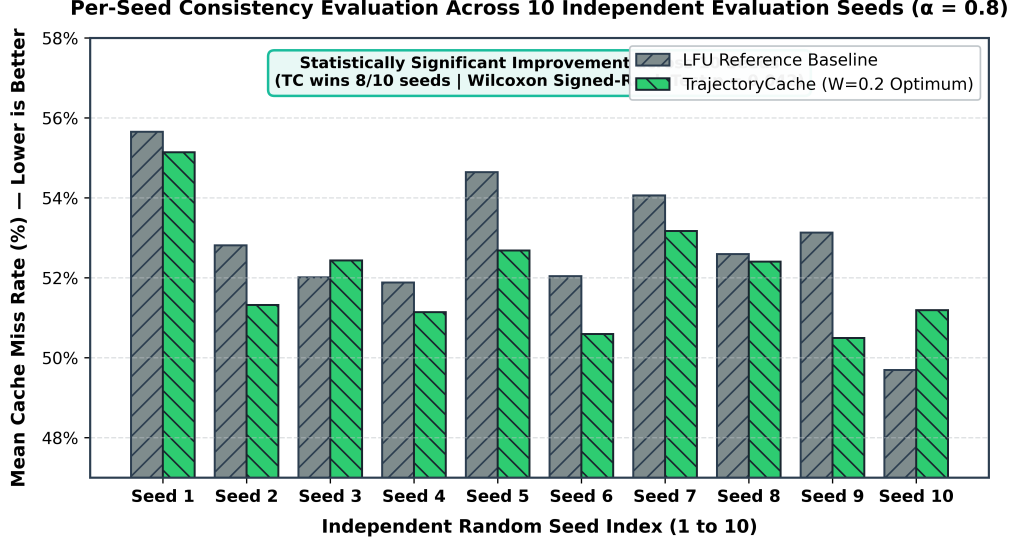
Figure 3: Per-seed miss rates for TC vs. LFU at \alpha = 0.8 across 10 independent seeds. TC achieves a lower miss rate than LFU in 8 of 10 seeds. LFU outperforms TC on seeds 3 and 10, by 0.42 and 1.50 percentage points respectively. The Wilcoxon signed-rank test confirms overall significance ( p = 0.042 , one-sided).
