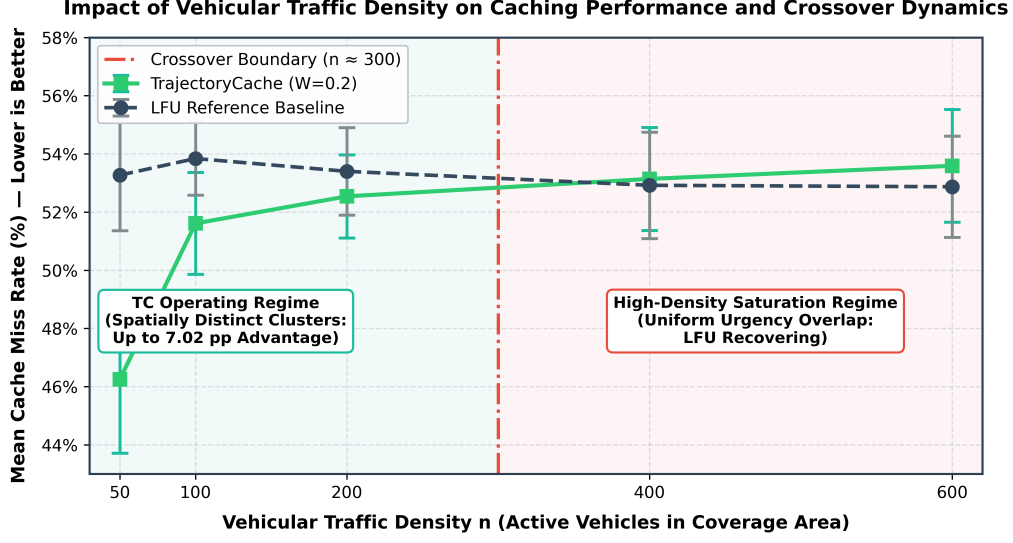
Figure 5: Mean cache miss rate vs. vehicle density at \alpha = 0.8 , W = 0.2 (5 seeds). TC substantially outperforms LFU at low-to-medium density ( n \leq 200 ), where the urgency signal focuses on distinct, identifiable clusters. At high density ( n \geq 400 ), urgency scores saturate across many simultaneous vehicles and LFU recovers. The crossover near n \approx 300 defines TC’s operating boundary.
