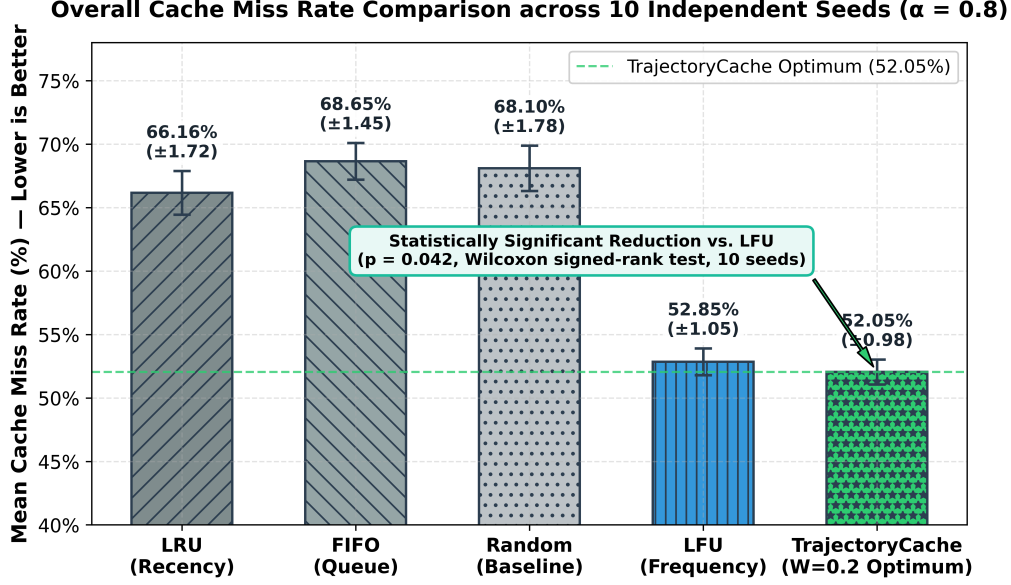
Figure 2: Mean cache miss rate across 10 seeds at \alpha = 0.8 . TC ( W = 0.2 ) achieves the lowest miss rate (52.05%). LFU is the strongest baseline (52.85%); TC’s 0.80 pp advantage over LFU is statistically significant ( p = 0.042 , Wilcoxon signed-rank test, one-sided).
