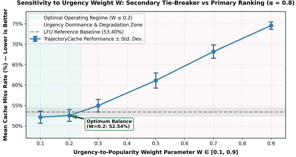
Figure 4: Mean cache miss rate vs. urgency weight W at \alpha = 0.8 (5 seeds). TC outperforms the LFU baseline only at W \leq 0.2 , confirming that the urgency term must augment, not override, the popularity signal. As W increases, the cache discards popular items based on transient spatial signals, causing progressive degradation.
