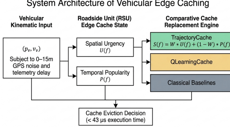
Figure 1: System architecture of the comparative vehicular edge caching framework. Vehicular kinematic input (p_v, v_v) subject to 0–15 m GNSS positioning noise and telemetry delay feeds into spatial urgency U(f) and temporal popularity P(f) extraction modules, which drive cache eviction decisions ( < 43 \mu\text{s} execution time) under closed-form rule-based TrajectoryCache, online reinforcement learning QLearningCache, and classical baselines.
