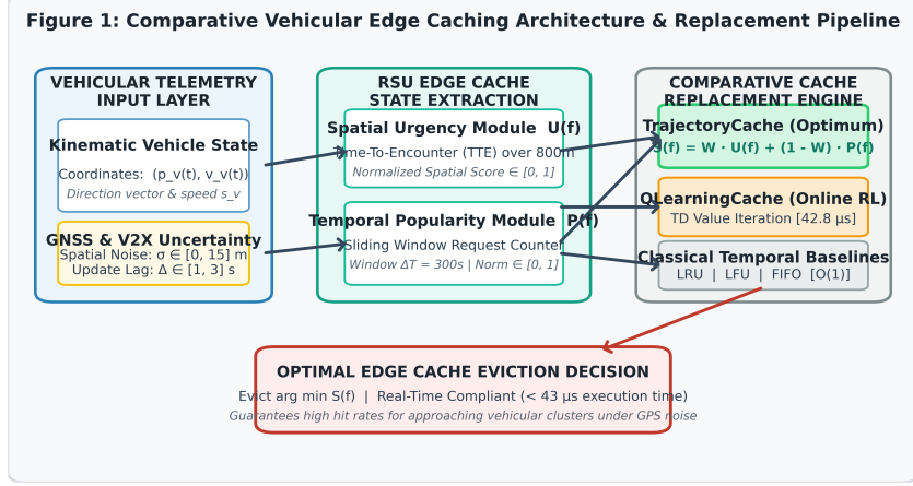
Figure 1: System architecture of the comparative vehicular edge caching framework. Vehicular kinematic input (p_v, v_v) subject to 0–15 m GNSS positioning noise and telemetry delay feeds into spatial urgency U(f) and temporal popularity P(f) extraction modules, which drive cache eviction decisions ( < 43 \mu\text{s} execution time) under closed-form rule-based TrajectoryCache, online reinforcement learning QLearningCache, and classical baselines.
