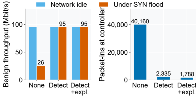
FIGURE 5. The emulated network under a randomized-source SYN flood. Left: benign iperf3 throughput with the network idle and during the flood, for each of the three conditions. Right: packet-in events reaching the controller over the same run. The conditions are abbreviated on the axes: “None” is the learning-switch controller with detection disabled, “Detect” adds the detector, and “Detect +expl” additionally attributes every admitted alert; Table 15 names them in full. Installing drop rules at the switch both preserves the benign transfer and removes most of the control-plane load the flood would otherwise impose.
