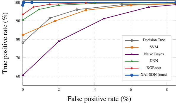
Figure 6: ROC curves for XAI-SDN and baselines on the binary DDoS detection task. XAI-SDN achieves AUC = 1.0000 with TPR = 99.99% at FPR = 0.054%.
