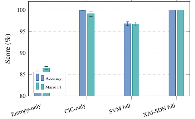
Figure 7: Feature ablation over the five archived seeds (mean \pm std). Neither feature family alone matches the full 88-dimensional configuration, and the RF outperforms an SVM given identical features.
