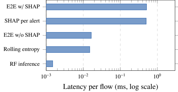
Figure 4: Latency contribution of each pipeline stage (log scale). Explanation generation dominates the per-flow budget when SHAP is invoked, motivating the alert-gated invocation policy of Algorithm 1.
