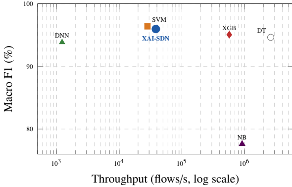
Figure 8: Macro F1 versus throughput under the controlled protocol. XAI-SDN occupies the operating region combining near-best F1 with practical throughput, and is the only marker backed by per-prediction explanations.
