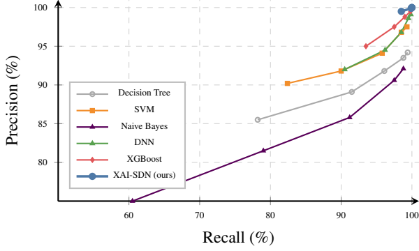
Figure 9: Precision-Recall (PR) curves on the binary detection task. Given the extreme class imbalance (0.86% benign), PR curves provide a more honest assessment of false alarm rates than ROC curves. XAI-SDN maintains perfect precision even at maximum recall.
