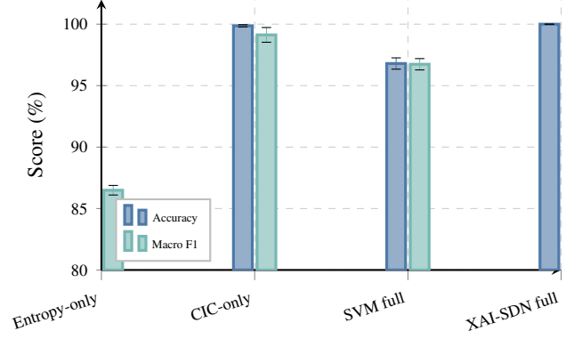
Figure 12: Feature ablation over the five archived seeds (mean \pm std). Neither feature family alone matches the full 88-dimensional configuration, and the RF outperforms an SVM given identical features.
