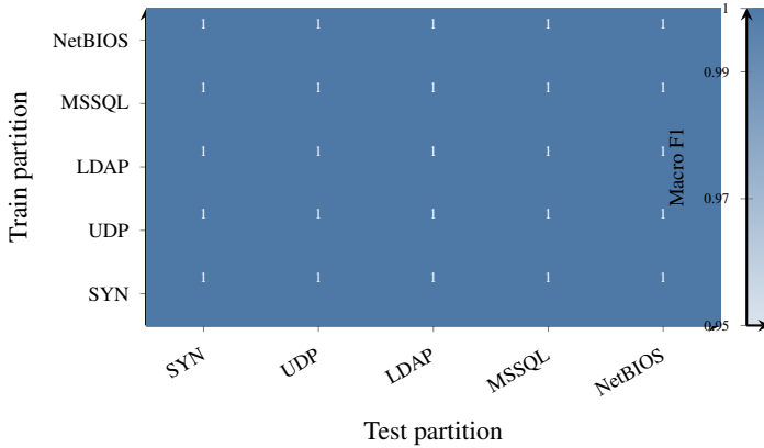
Figure 11: Cross-partition macro-F1 heatmap ( 5 \times 5 , train partition \times test partition). Every off-diagonal cell represents zero-shot transfer performance. XAI-SDN achieves \geq 1.000 F1 in all 25 cells, confirming attack-agnostic generalization across the five CIC-DDoS2019 attack vectors.
