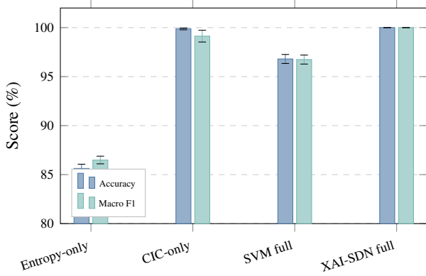
Figure 12: Feature ablation over the five archived seeds (mean \pm std). Neither feature family alone matches the full 88-dimensional configuration, and the RF outperforms an SVM given identical features.
