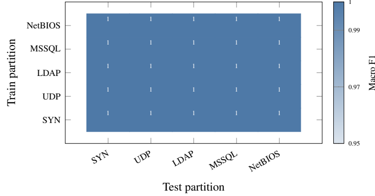
Figure 11: Cross-partition macro-F1 heatmap ( 5 \times 5 , train partition \times test partition). Every off-diagonal cell represents zero-shot transfer performance. XAI-SDN achieves \geq 1.000 F1 in all 25 cells, confirming attack-agnostic generalization across the five CIC-DDoS2019 attack vectors.
