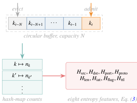
Figure 4: Rolling entropy engine. A circular buffer of the N most recent flow keys and a hash map of key multiplicities allow each admit/evict pair to update all eight entropy features in O(1) time, independent of N .
