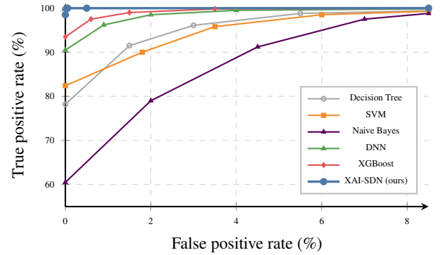
Figure 10: ROC curves for XAI-SDN and baselines on the binary DDoS detection task. XAI-SDN achieves AUC = 1.0000 with TPR = 99.99% at FPR = 0.054%.
