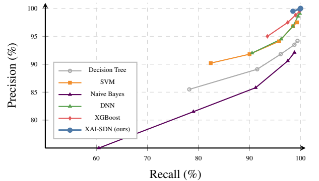
Figure 11: Precision-Recall (PR) curves on the binary detection task. Given the extreme class imbalance (0.86% benign), PR curves provide a more honest assessment of false alarm rates than ROC curves. XAI-SDN maintains perfect precision even at maximum recall.
