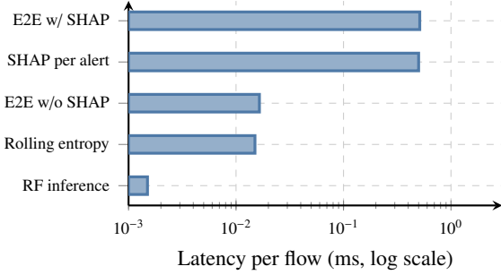
Figure 8: Latency contribution of each pipeline stage (log scale). Explanation generation dominates the per-flow budget when SHAP is invoked, motivating the alert-gated invocation policy of Algorithm 1.
