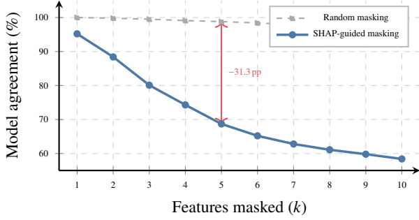
Figure 12: SHAP fidelity deletion curve (C1). Model agreement (% of test samples where the masked model matches the full model) under SHAP-guided feature masking (blue) vs. random masking (grey). At k = 5 the SHAP gap is -31.3 percentage points, confirming that SHAP attributions identify genuinely influential features rather than surface correlates.
