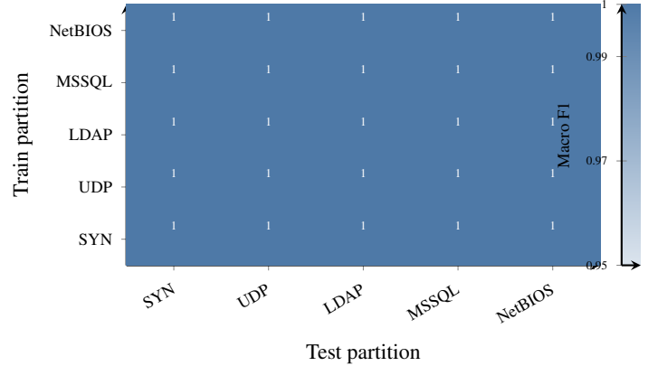
Figure 13: Cross-partition macro-F1 heatmap ( 5 \times 5 , train partition \times test partition). Every off-diagonal cell represents zero-shot transfer performance. XAI-SDN achieves \geq 1.000 F1 in all 25 cells, confirming attack-agnostic generalization across the five CIC-DDoS2019 attack vectors.
