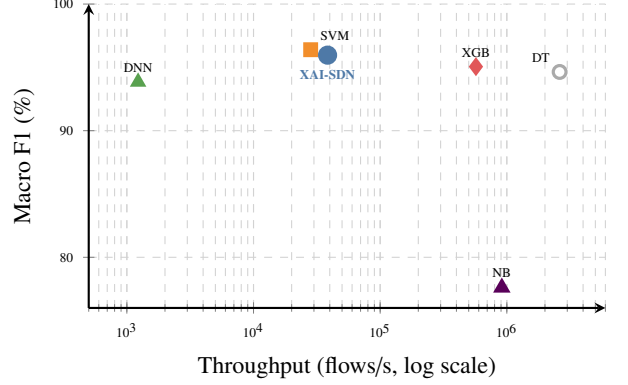
Figure 15: Macro F1 versus throughput under the controlled protocol. XAI-SDN occupies the operating region combining near-best F1 with practical throughput, and is the only marker backed by per-prediction explanations.
