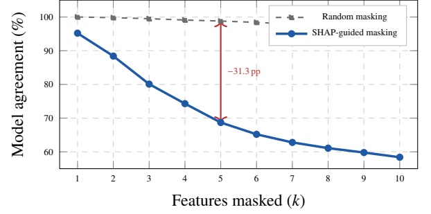
Figure 7: SHAP fidelity deletion curve (C1). Model agreement (% of test samples where the masked model matches the full model) under SHAP-guided feature masking (blue) vs. random masking (grey). At k = 5 the SHAP gap is -31.3 percentage points, confirming that SHAP attributions identify genuinely influential features rather than surface correlates.
