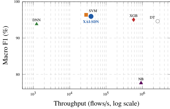
Figure 10: Macro F1 versus throughput under the controlled protocol. XAI-SDN occupies the operating region combining near-best F1 with practical throughput, and is the only marker backed by per-prediction explanations.
