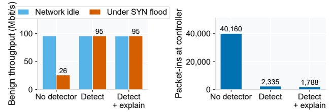
FIGURE 5. The emulated network under a randomized-source SYN flood. Left: benign iperf3 throughput with the network idle and during the flood, for each of the three conditions. Right: packet-in events reaching the controller over the same run. Installing drop rules at the switch both preserves the benign transfer and removes most of the control-plane load the flood would otherwise impose.
