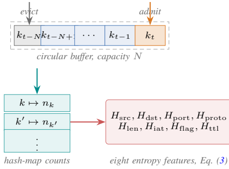
Fig. 2. Rolling entropy engine. A circular buffer of the N most recent flow keys and a hash map of key multiplicities allow each admit/evict pair to update all eight entropy features in \mathcal{O}(1) time, independent of N .
