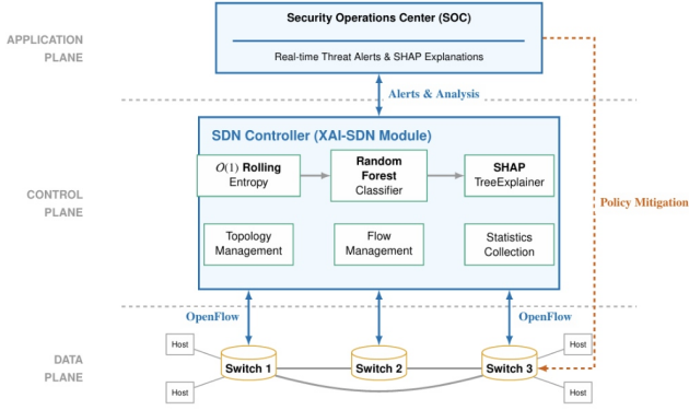
FIGURE 1. XAI-SDN system architecture. OpenFlow switches export flow statistics to the controller-embedded XAI-SDN module, which performs O(1) entropy-augmented feature extraction, Random Forest classification, and SHAP-based explanation generation. Detected DDoS events trigger alerts and policy updates; the dashed arrow represents the southbound policy-enforcement feedback loop.
