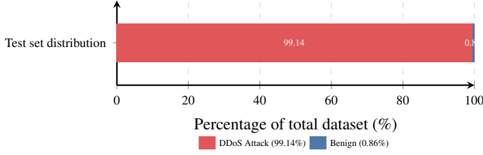
Figure 4: Extreme class imbalance in the CIC-DDoS2019 SYN test partition (1,077,798 flows). With less than 1% benign traffic, raw accuracy is not a reliable metric, necessitating the use of Macro F1 and Precision-Recall evaluation.
