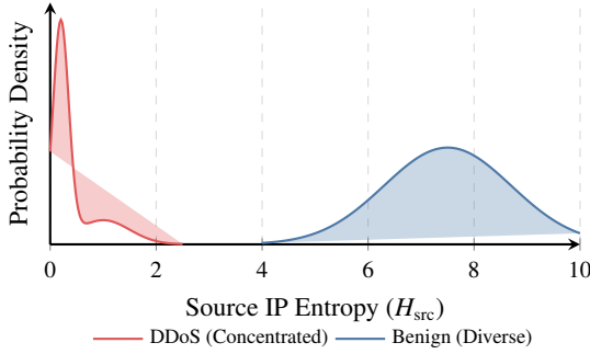
Figure 3: Conceptual distribution of Source IP Entropy ( H_{\text{src}} ). Benign traffic typically exhibits high entropy due to diverse source IP distributions in enterprise networks. Volumetric DDoS attacks, characterized by massive botnet concentration or spoofed subnets, exhibit a sharp density spike at near-zero entropy. This stark distributional divergence makes rolling entropy a highly discriminative feature prior to classifier ingestion.
