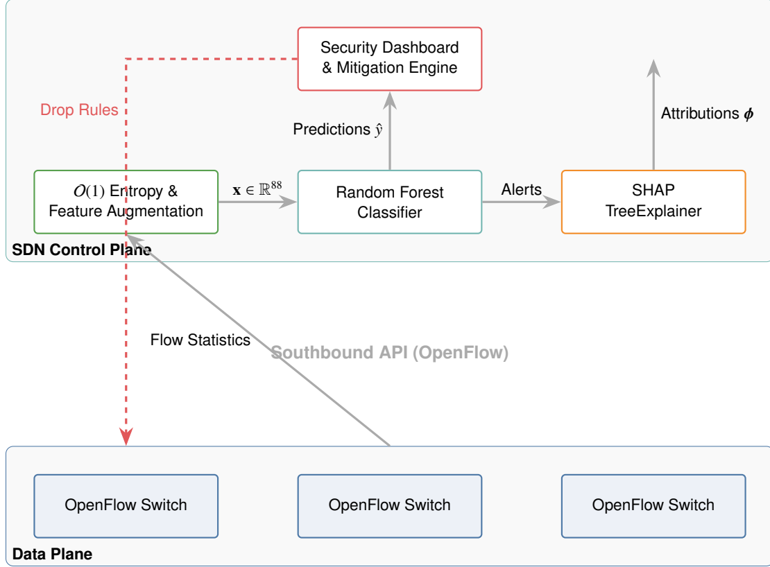
Figure 1: XAI-SDN system architecture. OpenFlow switches export flow statistics to the controller-embedded XAI-SDN module, which performs O(1) entropy-augmented feature extraction, Random Forest classification, and SHAP-based explanation generation. Detected DDoS events trigger alerts and policy updates; the dashed arrow represents the southbound policy-enforcement feedback loop.
