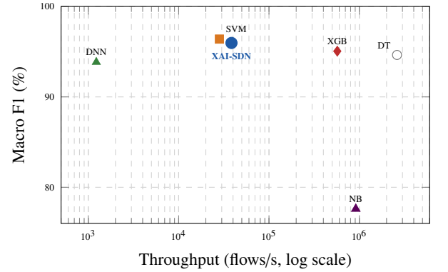
Figure 8: Macro F1 versus throughput under the controlled protocol. XAI-SDN occupies the operating region combining near-best F1 with practical throughput, and is the only marker backed by per-prediction explanations.
