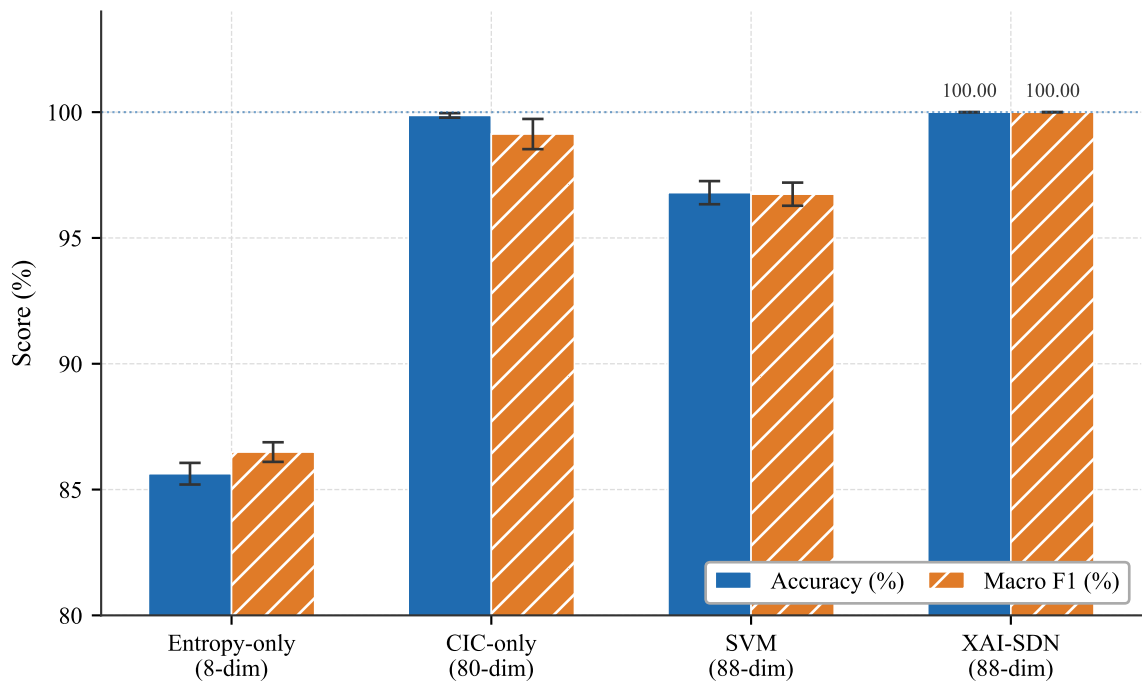
Feature ablation over the five archived seeds (mean \pm std). Neither feature family alone matches the full 88-dimensional configuration, and the RF outperforms an SVM given identical features.
