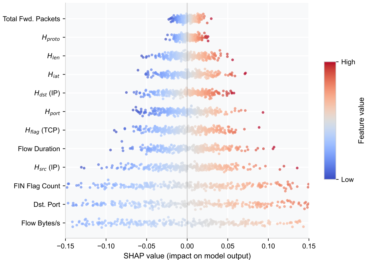
SHAP beeswarm plot illustrating the impact of feature values on model output. High values of specific entropy metrics and protocol flags strongly push the model toward a DDoS prediction.
