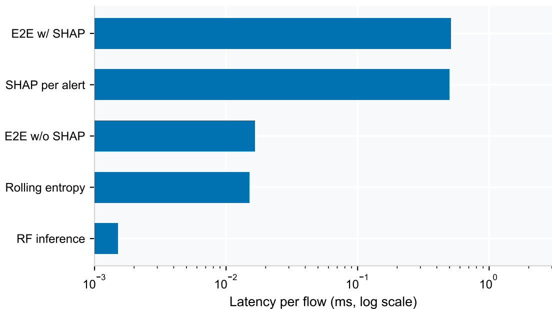
Latency contribution of each pipeline stage (log scale). Explanation generation dominates the per-flow budget when SHAP is invoked, motivating the alert-gated invocation policy of Algorithm ??.
