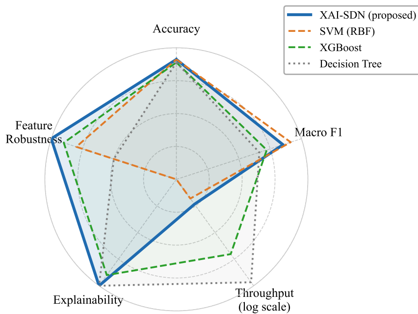
Multi-dimensional classifier comparison across five performance axes: Accuracy, Macro F1, log-scale Throughput, Explainability, and Feature Robustness. All axes are min-max normalized to [0, 1]. XAI-SDN (solid blue) covers the largest aggregate area, indicating the best overall balance. SVM lacks explainability; Decision Tree lacks feature robustness; XGBoost achieves high throughput but falls short on Explainability.
