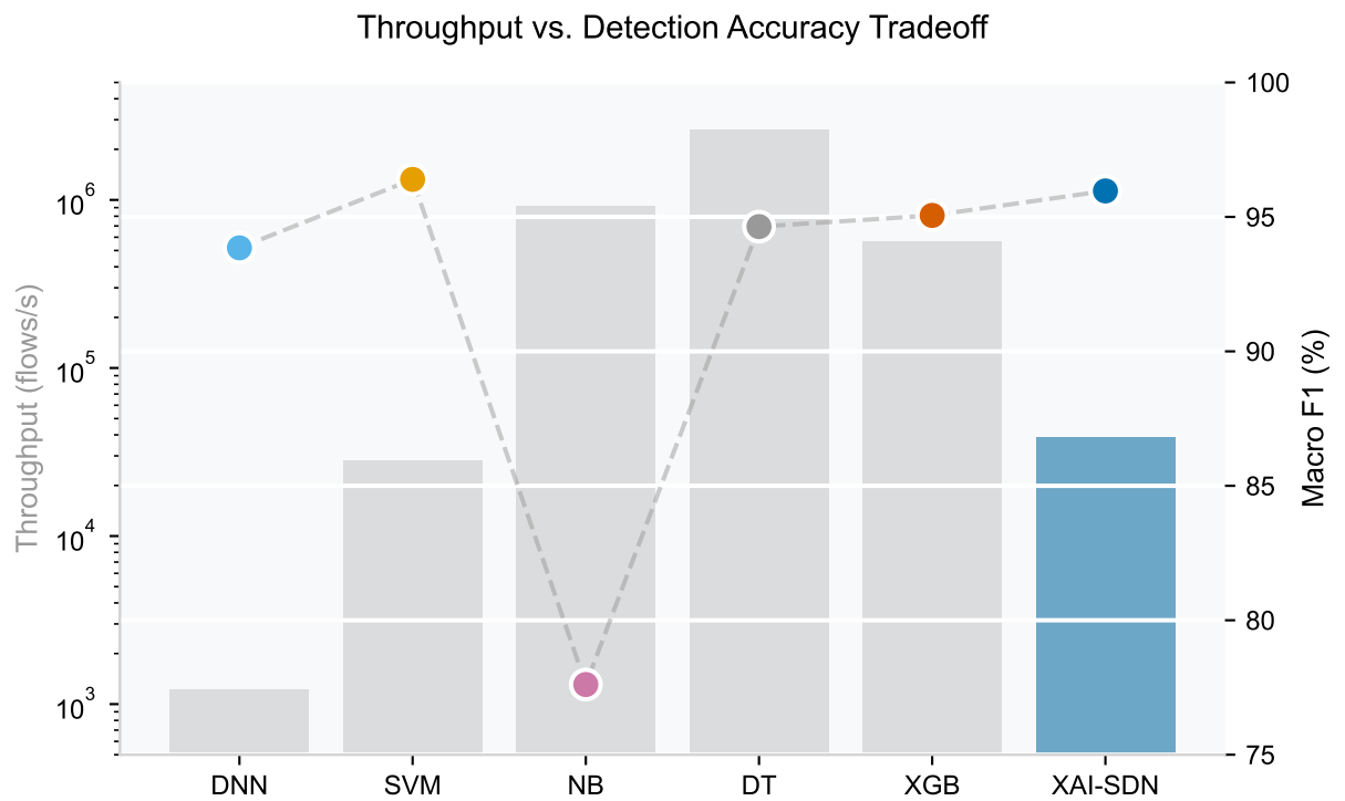
Macro F1 versus throughput under the controlled protocol. XAI-SDN occupies the operating region combining near-best F1 with practical throughput, and is the only marker backed by per-prediction explanations.
