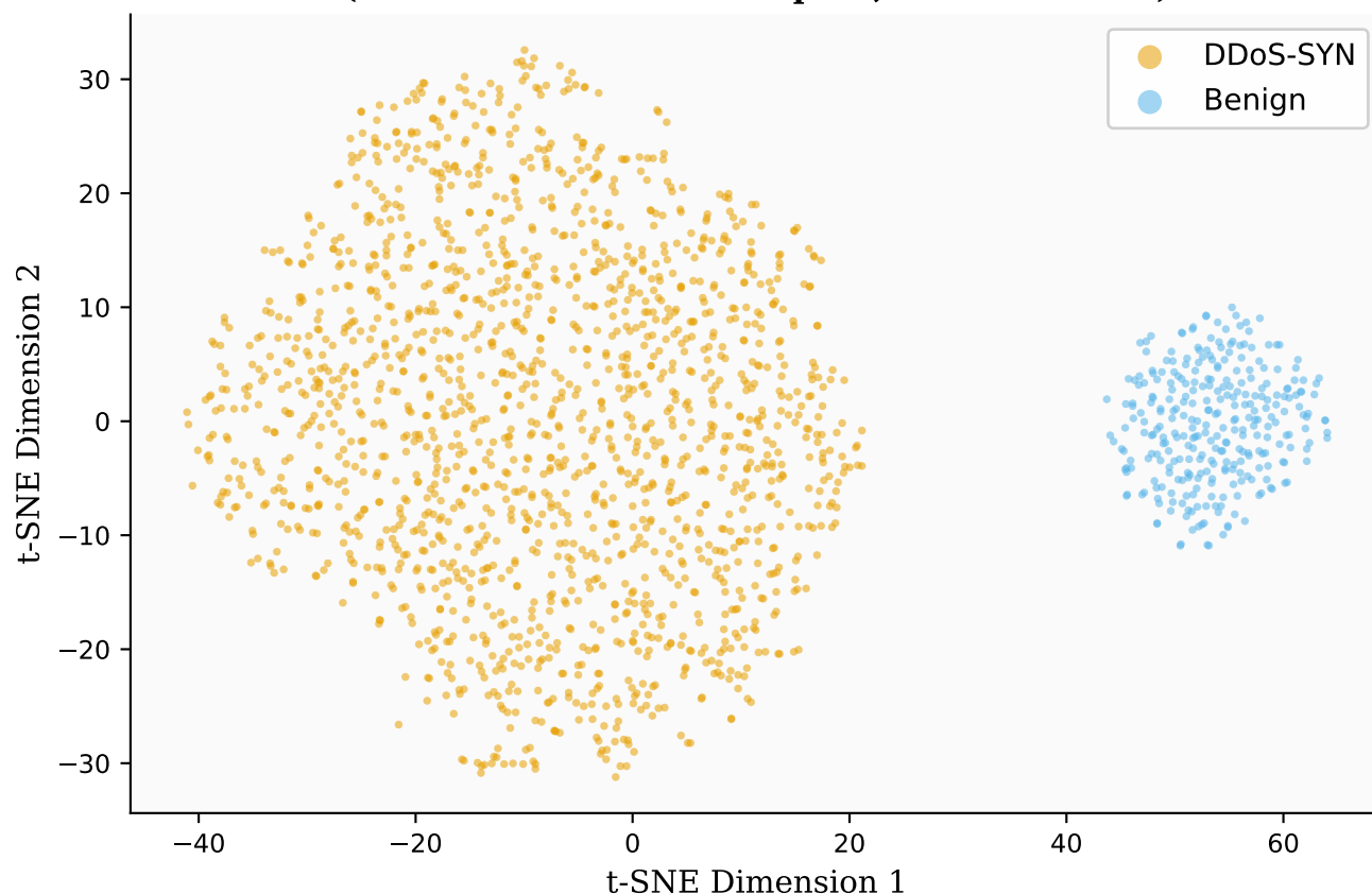
t-SNE Manifold: Benign vs. DDoS-SYN (88-dimensional feature space, CIC-DDoS2019)
