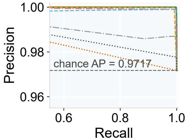
Precision-recall
