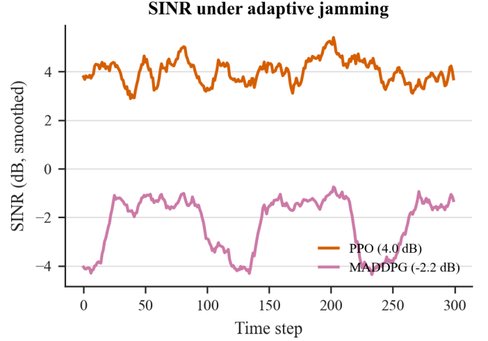
Fig. 3. Received SINR over time under adaptive jamming (smoothed).
