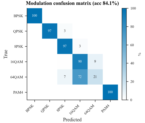
Fig. 7. Confusion matrix for six-class modulation recognition (% row-normalized).
