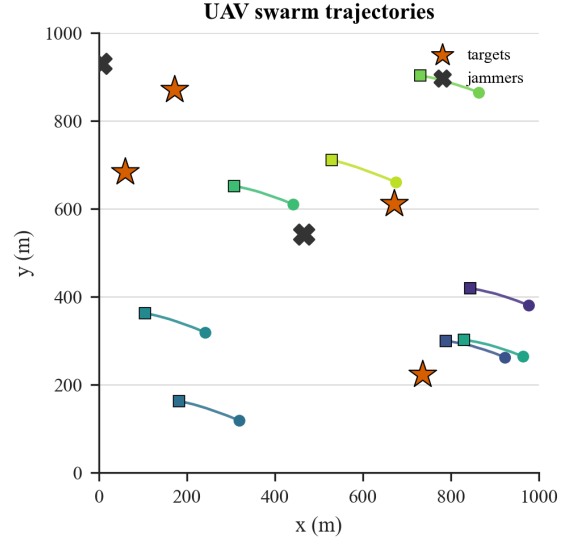
Fig. 3. Trajectories of the XM-MADRL swarm over one episode (circles: start, squares: end; stars: targets; crosses: jammers).
