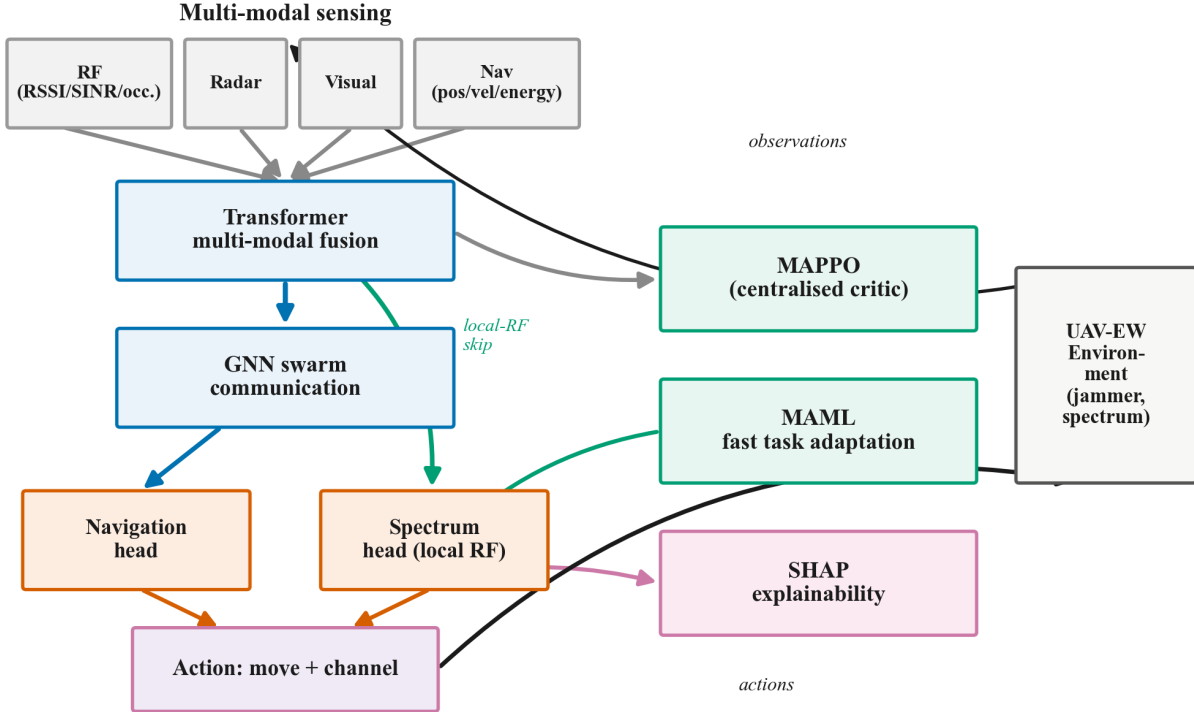
Fig. 1. The XM-MADRL framework. Multi-modal observations are fused by a Transformer and shared across the swarm by a GNN for coordinated navigation, while channel selection is driven by each agent’s local RF observations through a decoupled spectrum head (green “local-RF skip”). Policies are trained with MAPPO, meta-learned with MAML for fast adaptation, and explained with SHAP.
