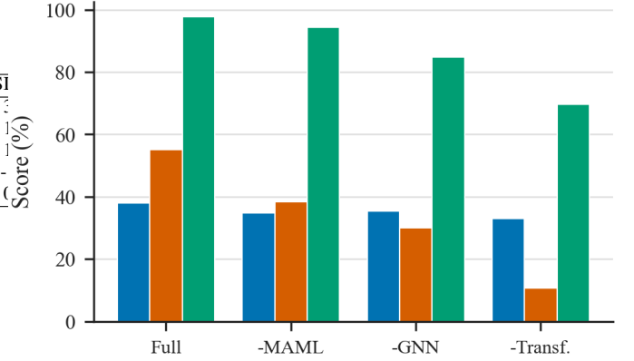
Ablation (component removal)
