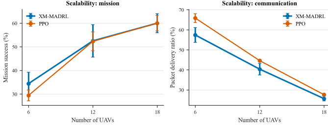
Fig. 8. Scalability of mission success and communication reliability with swarm size.
