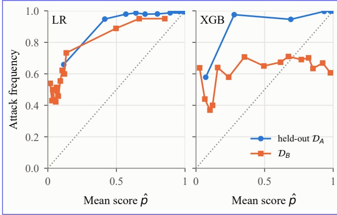
Fig. 7. Reliability diagrams for LR and XGB on held-out \mathcal{D}_A and on \mathcal{D}_B , fifteen equal-mass bins pooled over 20 split seeds.
