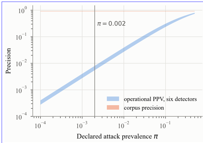
Fig. 6. Pooled operational precision against the declared attack prevalence \pi for the six radio-layer detectors, with the corpus precision for comparison. The vertical rule marks \pi = 0.002 .
