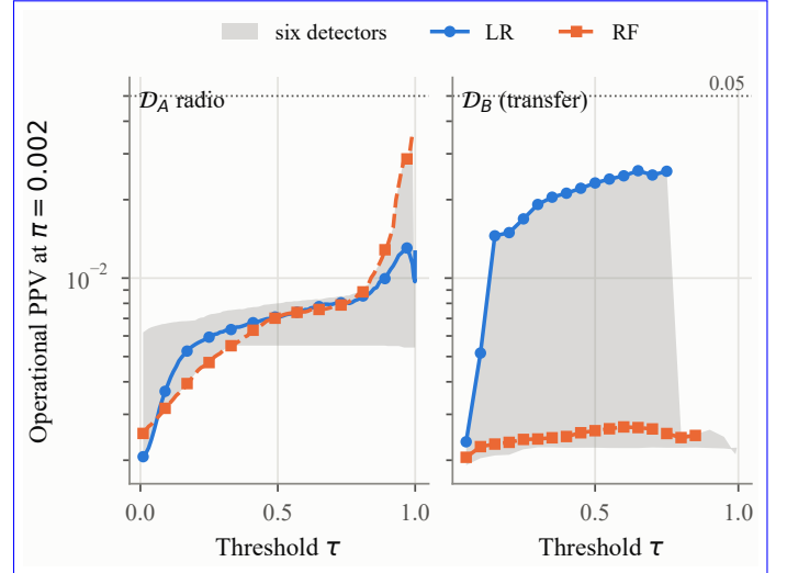
Fig. 5. Pooled operational precision at \pi = 0.002 against the decision threshold, radio layer and \mathcal{D}_B , for recall of at least 0.10.
