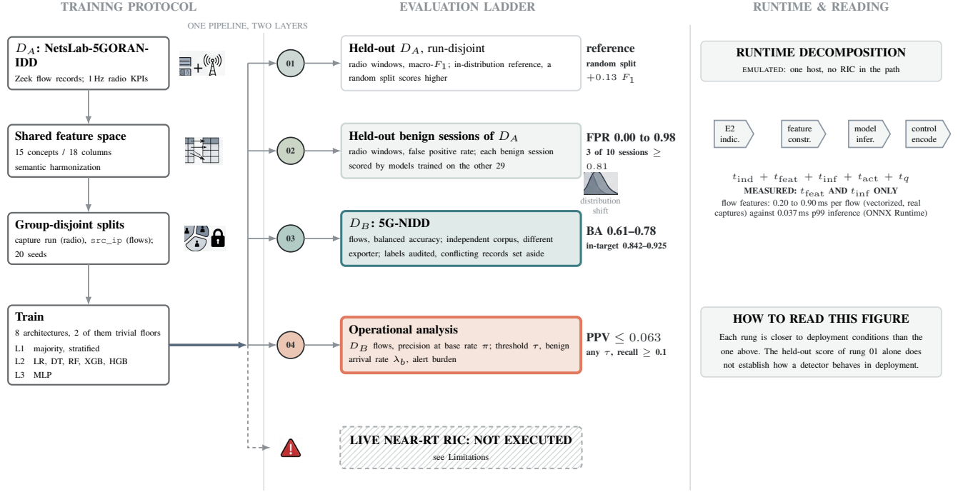
Fig. 2. Experimental pipeline. One pipeline, applied to two layers (radio windows for rungs 01 and 02, flows for 03 and 04), feeds an evaluation ladder whose rungs move closer to deployment conditions: a run-disjoint held-out split, held-out benign sessions, an independently collected corpus evaluated on its flows with consistent labels, and an operational analysis at a declared base rate. Each rung names its layer and metric; annotations give the measured values. The runtime panel is emulated on one host with no RIC in the path; the live-RIC arm was not executed.
