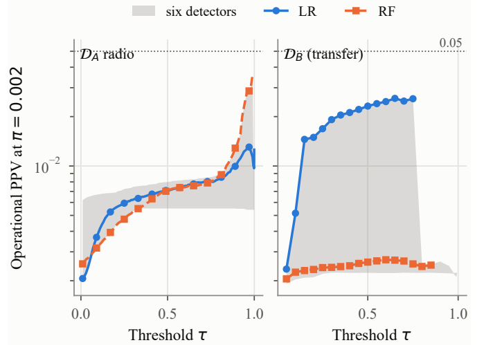
Fig. 5. Pooled operational precision at \pi = 0.002 against the decision threshold, radio layer and \mathcal{D}_B , for recall of at least 0.10.
