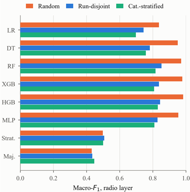
Fig. 3. Macro- F_1 on the \mathcal{D}_A radio layer under three protocols, mean over 20 split seeds. The random split inflates every supervised model; holding out runs while keeping every attack category in training does not remove the drop.
