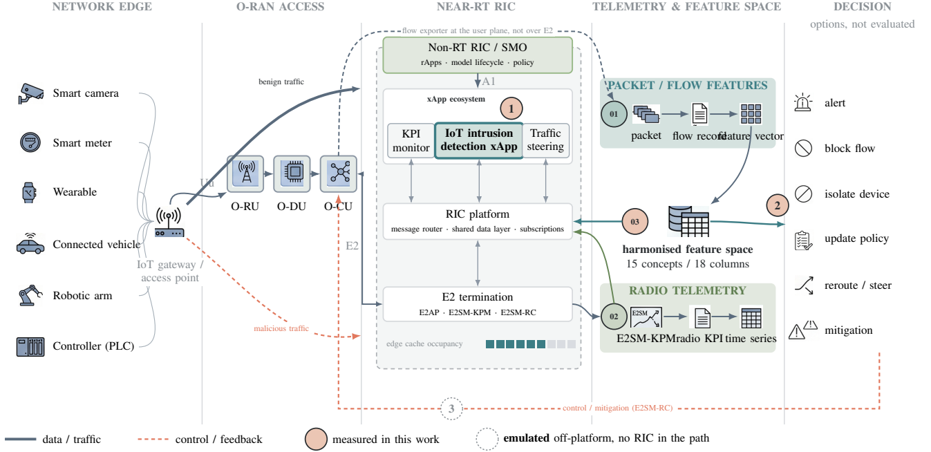
Fig. 1. Reference O-RAN edge deployment and the detection loop. The detection xApp in the near-real-time RIC receives radio telemetry over E2SM-KPM, and flow features from an exporter co-located with the user plane mapped onto the shared feature space. Numbered markers show what this paper measures: (1) generalization across corpora and (2) alert burden are measured on the corpora; (3) decision latency is emulated on one host with no RIC in the path. The mitigation actions on the right are the options E2SM-RC offers and are not evaluated.
