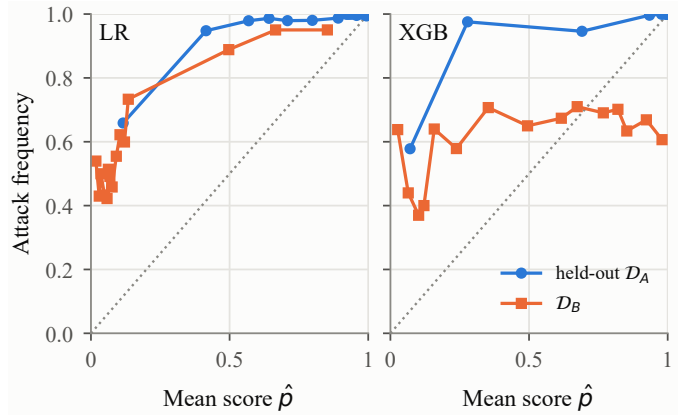
Fig. 7. Reliability diagrams for LR and XGB on held-out \mathcal{D}_A and on \mathcal{D}_B , fifteen equal-mass bins pooled over 20 split seeds.
