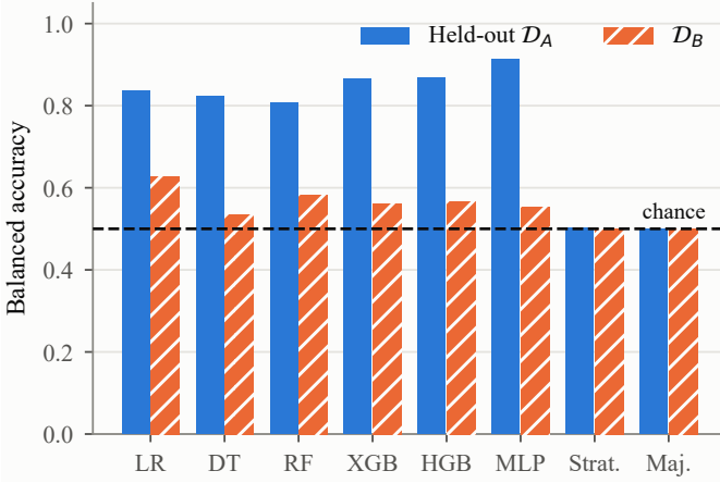
Fig. 4. Balanced accuracy on held-out \mathcal{D}_A and on \mathcal{D}_B , mean over 20 split seeds. The dashed line is chance (0.5), where both trivial baselines sit on both corpora.
