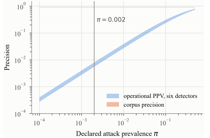
Fig. 6. Pooled operational precision against the declared attack prevalence \pi for the six radio-layer detectors, with the corpus precision for comparison. The vertical rule marks \pi = 0.002 .
