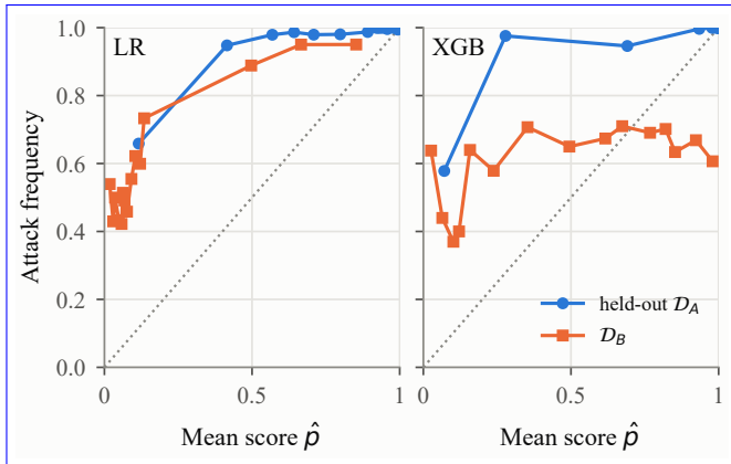
FIGURE 7. Reliability diagrams for LR and XGB on held-out \mathcal{D}_A and on \mathcal{D}_B , fifteen equal-mass bins pooled over 20 split seeds.
