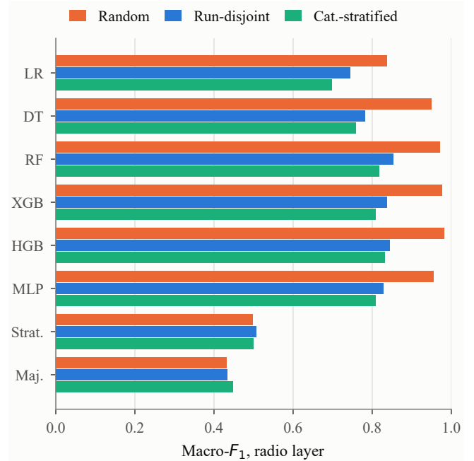
FIGURE 3. Macro- F_1 on the \mathcal{D}_A radio layer under three protocols, mean over 20 split seeds. The random split inflates every supervised model; holding out runs while keeping every attack category in training does not remove the drop.
