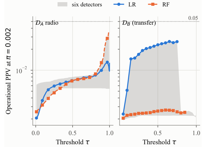
FIGURE 5. Pooled operational precision at \pi = 0.002 against the decision threshold, radio layer and \mathcal{D}_B , for recall of at least 0.10.
