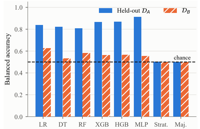
FIGURE 4. Balanced accuracy on held-out \mathcal{D}_A and on \mathcal{D}_B , mean over 20 split seeds. The dashed line is chance (0.5), where both trivial baselines sit on both corpora.
